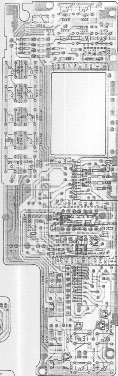
CONTROL UNIT (X53-1460 XX) 12 : K,M 52 : T 62 : W Foil side view
