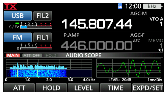
AUDIO SCOPE-Bildschirm
